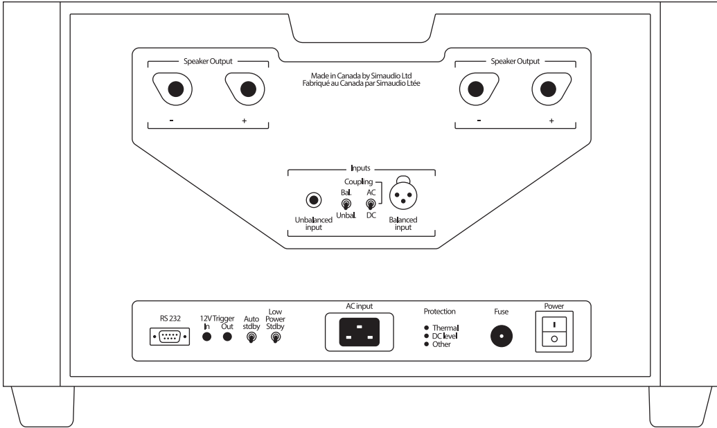
Figure 1: 888 Backpanel
