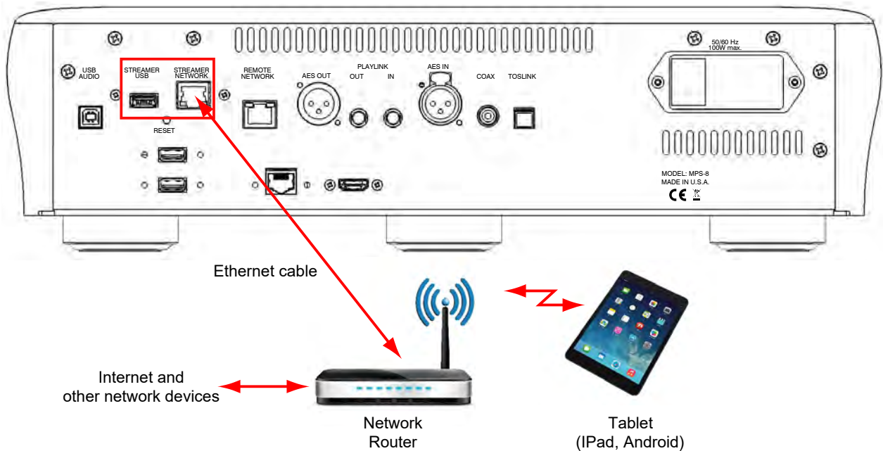
Stream-X2 connections on back panel of MPT-8
