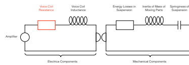
Figure 20.1: A simplified version of the actual electrical and electrical analogies of mechanical components in a loudspeaker driver.
