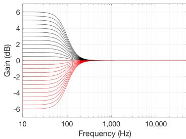
Figure 5.42: Magnitude Responses, low-shelving filter: F_c = 100 Hz, Gain varied from -6.0 to +6.0 dB, Q = 0.7 .
