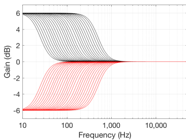
Figure 5.43: Magnitude Responses, low-shelving filter: F_c varied from 32 Hz to 500 Hz., Gain = \pm 6 dB, Q = 0.7 .
