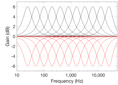
Figure 5.46: Magnitude Responses, Peaking filters: Examples of F_c varied from 25 Hz to 25 kHz on one-octave centres, Gain = \pm 6 dB, Q = 1 .
