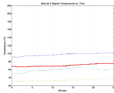
Figure 20.3: The temperatures of the magnets of the loudspeaker drivers in a BeoLab 5 as a result of playing pop music at full volume. The X-axis is the time in minutes.
