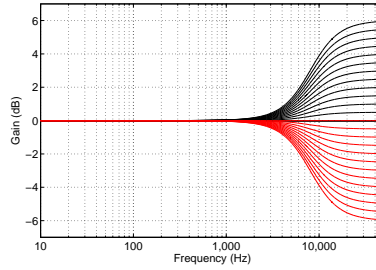
Figure 5.35: Magnitude Responses, Treble controller. Note that this filter is applied to both loudspeakers simultaneously.
