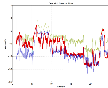
Figure 20.6: The gains (in dB) applied to the signals sent to the drivers in a BeoLab 5 as a result of playing pop music at full volume. The X-axis is the time in minutes.
