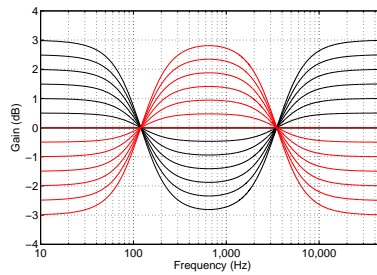
Figure 5.40: Magnitude Responses, Sound Enhance controller. Note that this filter is applied to both loudspeakers simultaneously. Black curves show the result for positive slider values, red curves show negative slider values.
