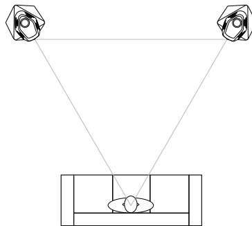
Figure 5.2: A “perfect” loudspeaker configuration with BeoLab 90’s. Both loudspeakers are aimed at the listening position. The distance from the listening position to each loudspeaker is the same as the distance between the two loudspeakers. For more detailed information on loudspeaker configuration, see Appendix 1: Recommendations for Critical Listening
