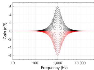
Figure 5.45: Magnitude Responses, Peaking filter: F_c = 100 Hz, Gain varied from -6.0 to +6.0 dB, Q = 1 .
