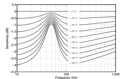
Figure 20.4: Sensitivity of BeoLab 90's front woofer vs. the change in temperature of its voice coil.
