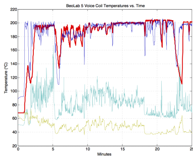
Figure 20.2: The temperatures (in °C) of the voice coils of the drivers in a BeoLab 5 as a result of playing pop music at full volume. The X-axis is the time in minutes.
