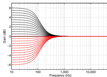
Figure 5.36: Magnitude Responses, Bass controller. Note that this filter is applied to both loudspeakers simultaneously.
