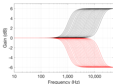
Figure 5.49: Magnitude Responses, high-shelving filter: F_c varied from 1 kHz to 16 kHz, Gain = \pm 6 dB, Q = 0.7 .
