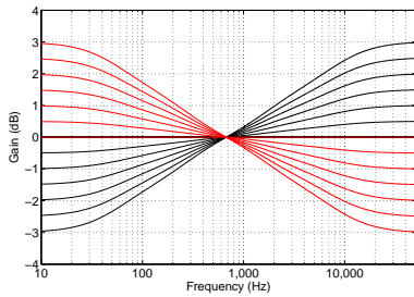
Figure 5.39: Magnitude Responses, Frequency Tilt controller. Note that this filter is applied to both loudspeakers simultaneously. Black curves show the result for positive slider values, red curves show negative slider values.
