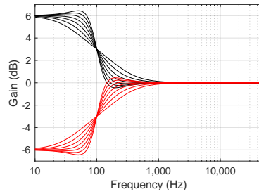
Figure 5.44: Magnitude Responses, low-shelving filter: F_c = 100 Hz, Gain = \pm 6 dB, Q varied from 0.4 to 1. Note that, for Q values greater than 0.7, there is an overshoot in the magnitude response. For a monotonically increasing (or decreasing) response, the Q should not be set to a value greater than 0.7.
