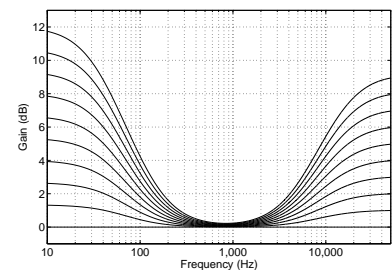
Figure 5.38: Magnitude responses of the loudness function at various settings of the volume control.
