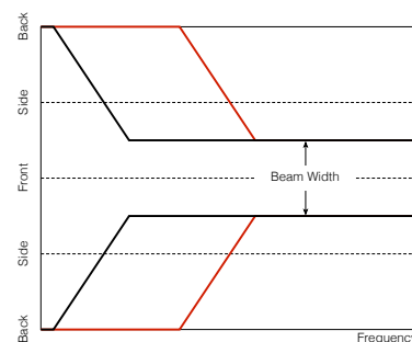
Figure 5.37: Conceptual plot showing the relationship between Latency Mode and a Narrow Beam Width over frequency. The black curve shows a High latency mode. The red curve shows a low latency mode. Note that the high frequency beam width is the same for both latency modes. Only the beam width of the low frequency bands widen for lower latencies.
