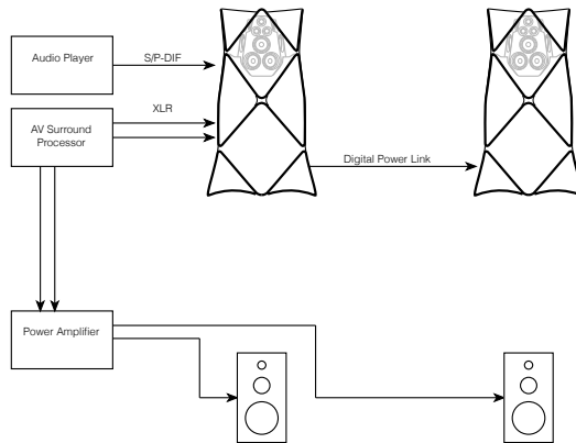
Figure 5.52: An example of a pair of BeoLab 90's connected to two third-party sources: an AV Surround Processor using XLR and a separate audio player using S/PDIF. Note that, in this case, the latency of the BeoLab 90's must be carefully managed in the setup of the loudspeakers and the AV Surround Processor in order to ensure that the multichannel system is behaving correctly.
