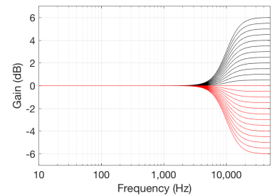
Figure 5.48: Magnitude Responses, high-shelving filter: F_c = 10 kHz, Gain varied from -6.0 to +6.0 dB, Q = 0.7 . Note that this filter is applied to both loudspeakers simultaneously.
